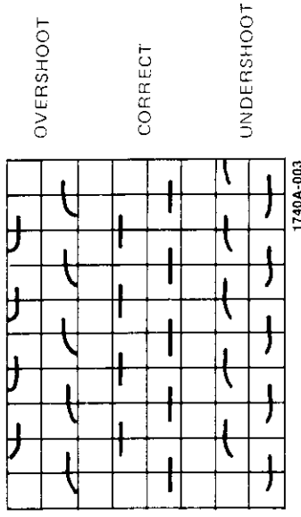
Figure 4. Probe Compensation
