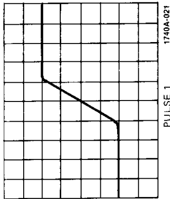
Figure 17b. Time Interval Measurement Using Delayed Time Base - Pulse 1
